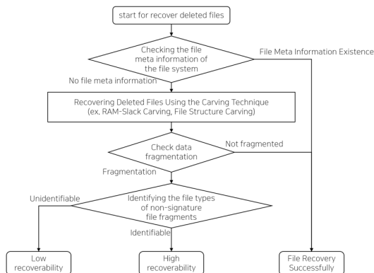
Fig. 1. File Recovery Flow
